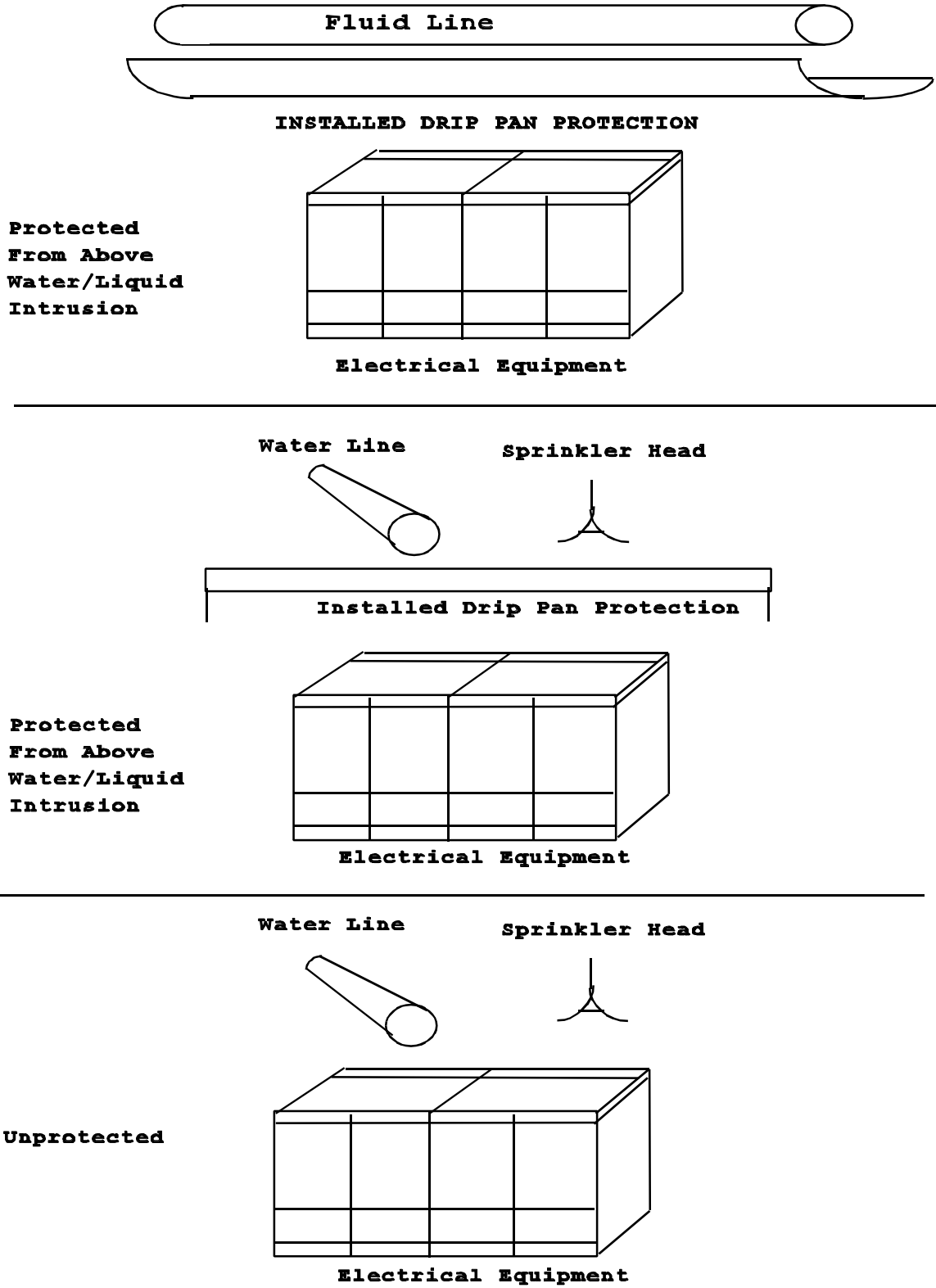
Figure 1. PROTECTED AND UNPROTECTED EQUIPMENT INSTALLATIONS
