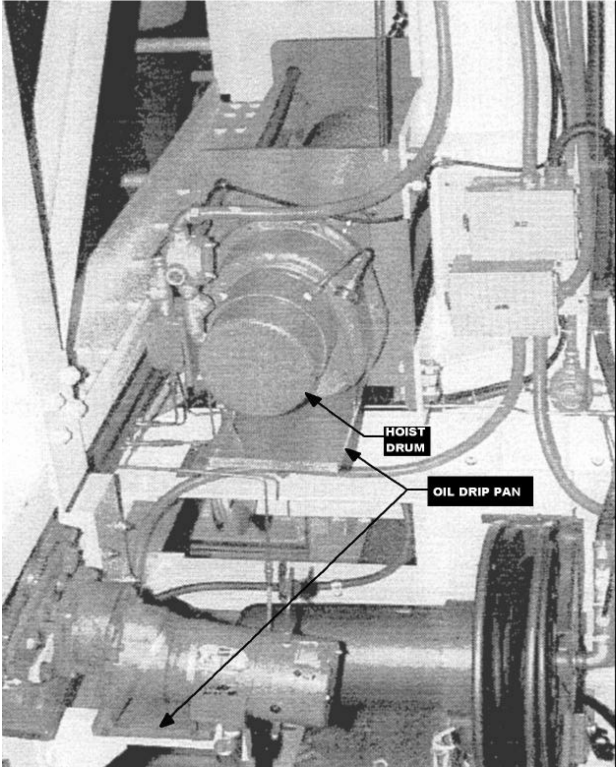
Figure 2. Placement of Oil Drip Pans
