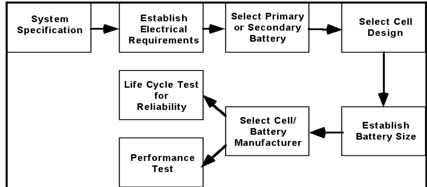
Figure 4. Typical Battery Selection Flow chart
