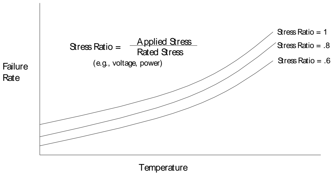
Figure 1. Piece-part Failure Rate vs. Temperature
